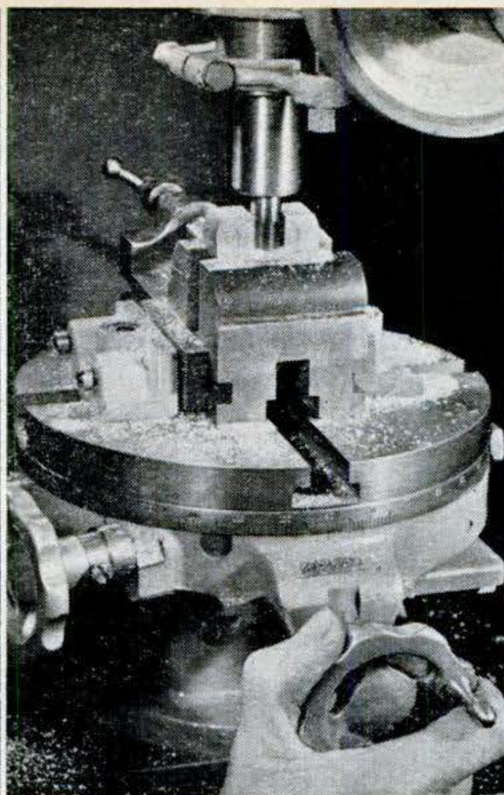
END MILLING a \frac{1}{2} " slot in aluminum. Keyways are similarly cut in shaft ends. Cross-feed of milling table is used to move work.
